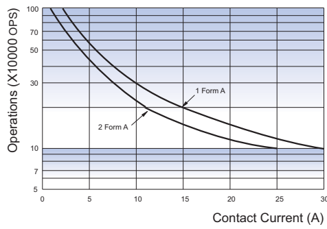
ENDURANCE CURVE
