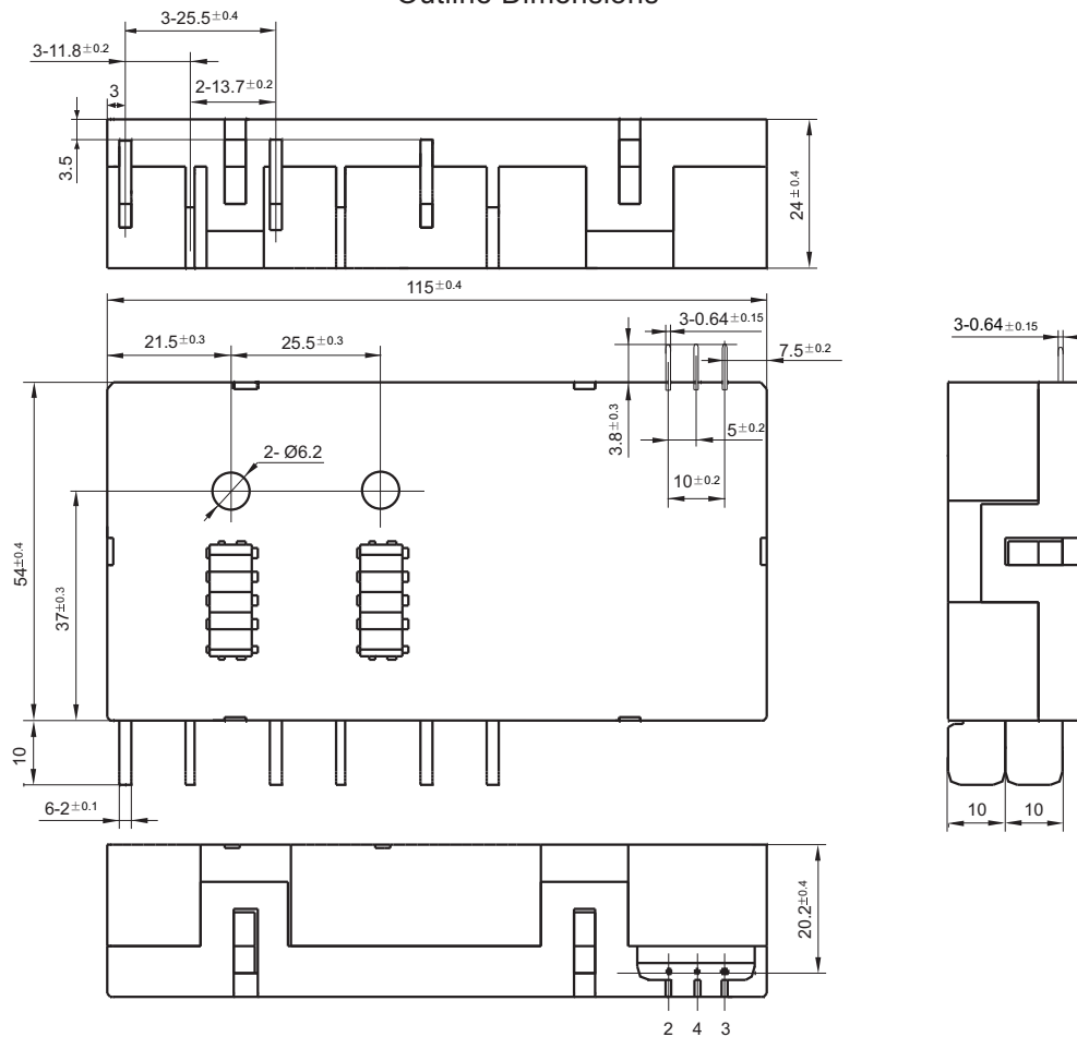
Outline Dimensions
